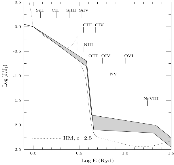
Fig. 2. The ionizing spectrum corresponding to the ionization state observed in the z_{\text{abs}} = 2.5745 system (HE1347–2457) is one from the shaded area. For comparison the intergalactic ionizing spectrum at z = 2.5 modeled by Haardt & Madau (1996) is shown by the dotted line. The spectra are normalized so that J_\nu(h\nu = 1 \text{ Ryd}) = 1 . The positions of ionization thresholds of different ions are indicated by tick marks.
