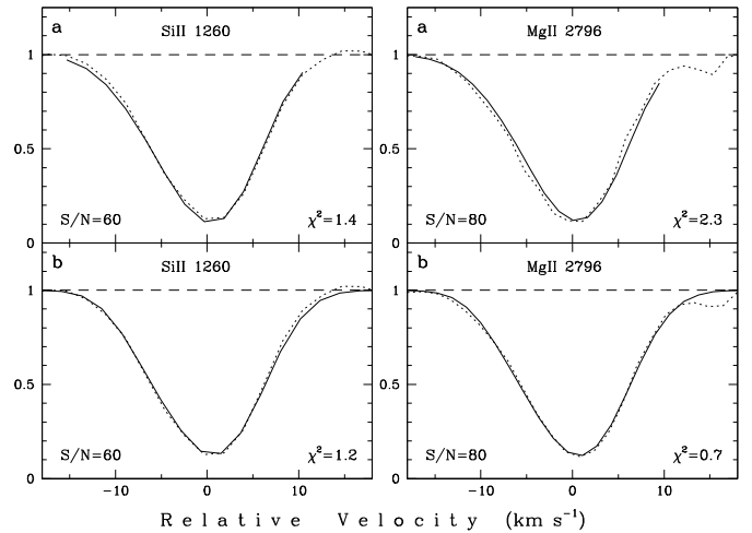
Fig. 5. Mg II in the z_{\text{abs}} = 1.7529 system (HE1347–2457). Panel a): observed (points) and synthetic (solid lines) profiles when Mg II lines are centered using the solar composition of the isotopes ^{24}\text{Mg}:^{25}\text{Mg}:^{26}\text{Mg} = 79:10:11 . Panel b): observed (points) and synthetic (solid lines) profiles when Mg II lines are shifted by 0.6 \text{ km s}^{-1} which corresponds to the inverse isotope composition ^{24}\text{Mg}:^{25}\text{Mg}:^{26}\text{Mg} = 11:10:79 . The corresponding signal-to-noise (S/N) mean value per resolution element at the continuum level and the obtained \chi^2_{\text{min}} per degree of freedom are shown.
