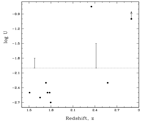
Fig. 16. Ionization parameter \log U estimated from metal-rich absorbers with redshifts 1.5 < z < 2.9 (see Table 2). The dashed line separates absorbers with low and high U -values.
