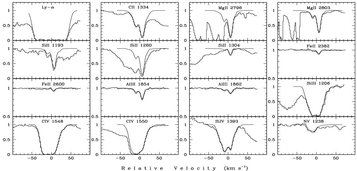
Fig. 10. Same as Fig. 1 but for the z_{\text{abs}} = 1.7315 system (HE0151–4326).
