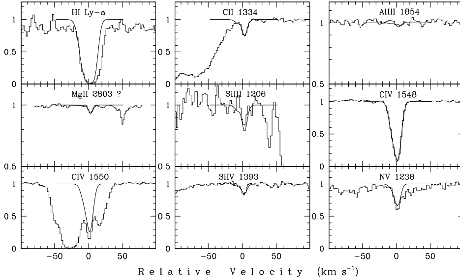
Fig. 14. Same as Fig. 1 but for the z_{\text{abs}} = 1.5770 system (HE0001–2340). Identification of the Mg II \lambda 2803 line is putative since the stronger component Mg II \lambda 2796 is blended with telluric absorption.
