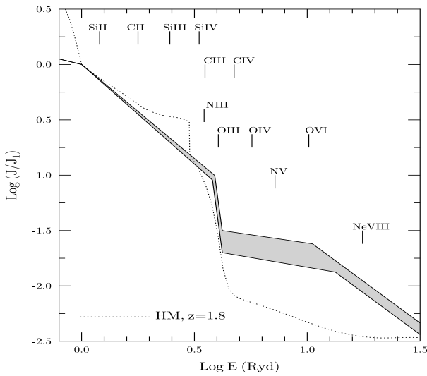
Fig. 4. Same as Fig. 2 but for the z_{\text{abs}} = 1.7529 system (HE1347–2457).
