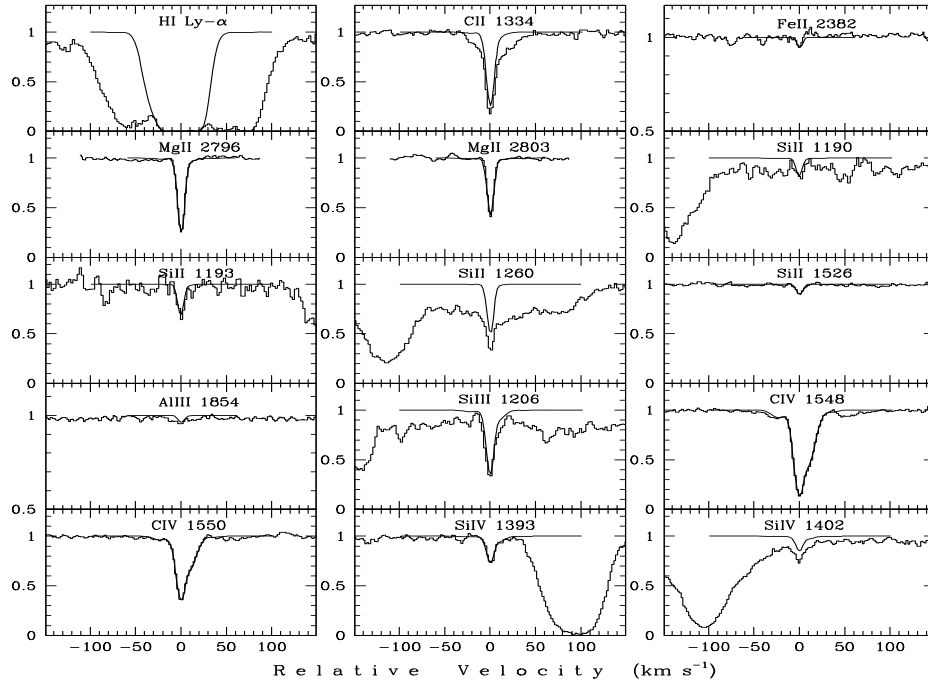
Fig. 12. Same as Fig. 1 but for the z_{\text{abs}} = 1.65136 system (HE0001–2340).
