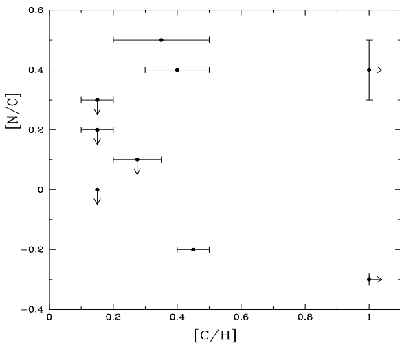
Fig. 15. Relative ratio [N/C] versus metallicity index [C/H] for metal-rich absorbers (see Table 3).
