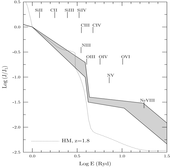
Fig. 11. Same as Fig. 2 but for the z_{\text{abs}} = 1.7315 system (HE0151–4326).
