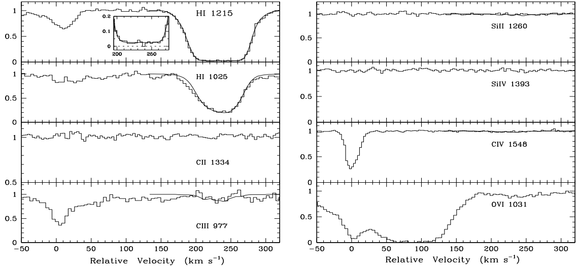
Fig. 9. Same as Fig. 1 but for the complex absorption system at z_{\text{abs}} = 2.3520 towards Q0329–385. The subsystem at v = 0 \text{ km s}^{-1} is described in Paper I, Sect. 2.4. The subsystem at v = 230 \text{ km s}^{-1} has z_{\text{abs}} = 2.3545 .
