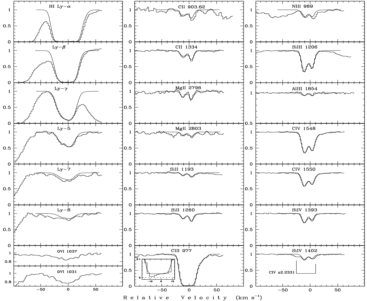
Fig. 1. Hydrogen and metal absorption lines from the z_{\text{abs}} = 2.5745 system towards HE1347–2457 (solid-line histograms). The vertical axis is normalized intensities. The zero radial velocity is fixed at z = 2.5745 . Synthetic profiles are plotted by the smooth curves. The wide profiles of the O VI \lambda\lambda 1031, 1037 lines show that the narrower line metal-rich system is embedded in a hot gas (seen also in H I Ly- \alpha and Ly- \beta lines as a difference between the observed and synthetic profiles). The insert in panel C III \lambda 977 demonstrates a non-zero residual intensity at the line center. The identified blend is marked in panel Si IV \lambda 1402 .
