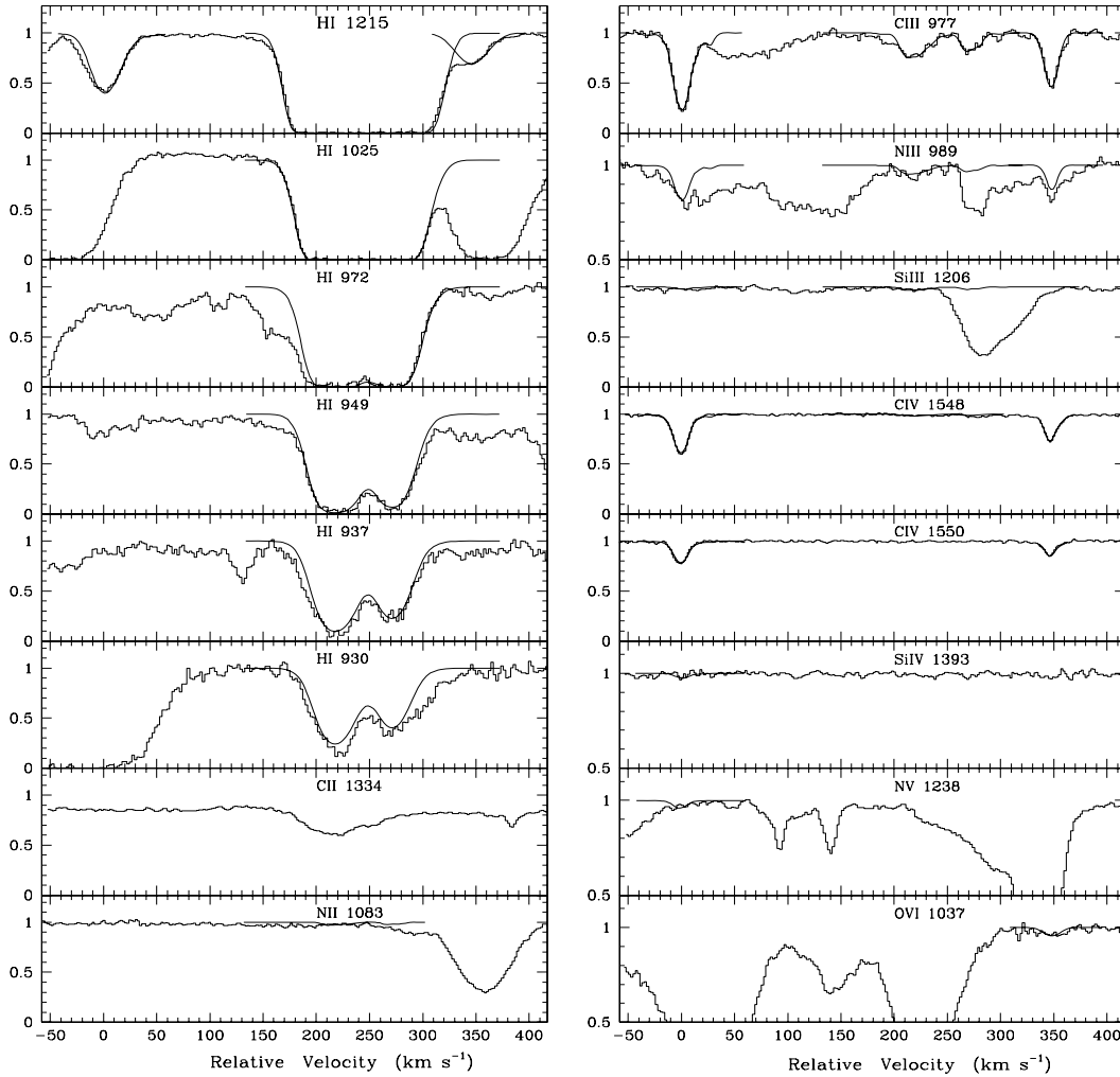
Fig. 8. Same as Fig. 1 but for the complex absorption system at z_{\text{abs}} = 2.4158 towards HE0151–4326. Three subcomponents cover the ranges: -30 < v < 40 \text{ km s}^{-1} (A), 140 < v < 340 \text{ km s}^{-1} (B), and 300 < v < 380 \text{ km s}^{-1} (C).
