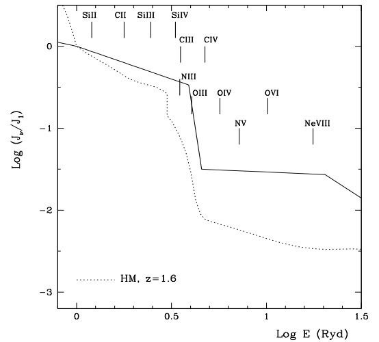
Fig. 13. The ionizing spectrum (solid line) corresponding to the ionization state observed in the z_{\text{abs}} = 1.65136 system (HE0001–2340). The intergalactic ionizing spectrum at z = 1.6 modeled by Haardt & Madau (1996) is shown by the dotted line. The spectra are normalized as in Fig. 2.
