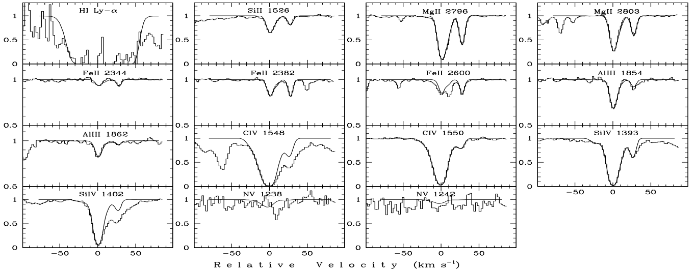
Fig. 6. Same as Fig. 1 but for the z_{\text{abs}} = 1.5080 system (HE1347–2457).
