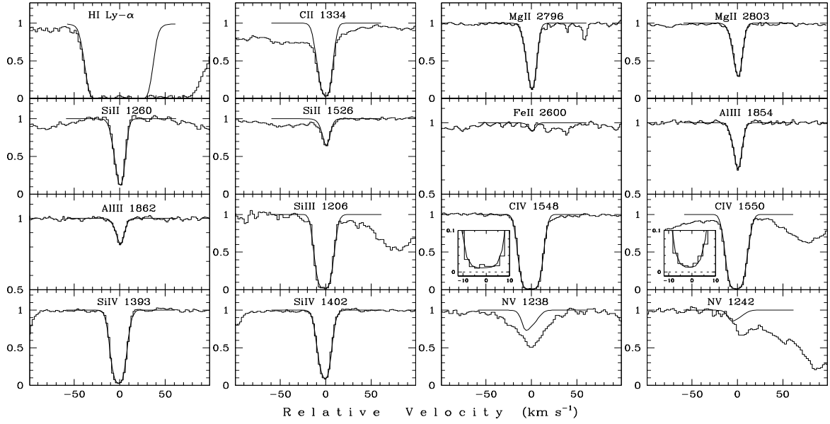
Fig. 3. Same as Fig. 1 but for the z_{\text{abs}} = 1.7529 system (HE1347–2457). The vertical axis is normalized intensities. The zero radial velocity is fixed at z = 1.7529 .
