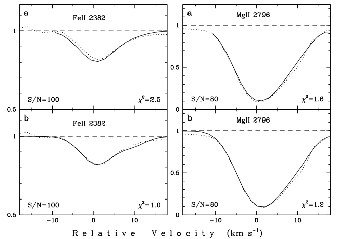
Fig. 7. Same as Fig. 5 but for the z_{\text{abs}} = 1.5080 system (HE1347–2457). In contrast to Fig. 5a where both lines Si II and Mg II are equivalently strong, here Fe II is significantly weaker than Mg II and, hence, the weight of Mg II dominates in the minimization of the objective function leading to a prominent shift of the Fe II line.
