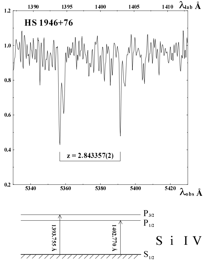
Fig. 1. Fine doublet splitting from quasar spectra
