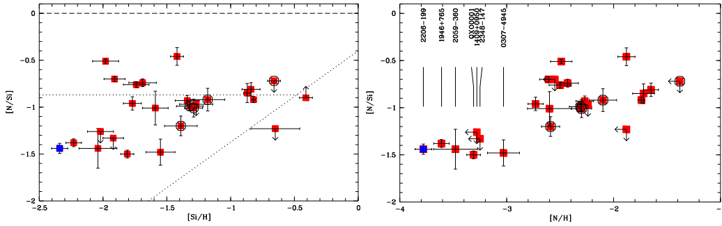
Fig. 2. Left panel: [N/Si] versus [Si/H] in DLAs. Bold octagons indicate our new DLA measurements. The blue point is our redetermination for z_{\text{abs}}=2.076 DLA in Q2206-199. Dotted lines are empirical representations of the secondary and primary N production. The horizontal line (primary) is plotted at the mean [N/Si] value in DLAs. Right panel: [N/Si] versus [N/H] in DLAs, where measurements seems to be separated in two groups. Bold octagons indicate our new DLA measurements. The blue point is our redetermination for z_{\text{abs}}=2.076 DLA in Q2206-199.
