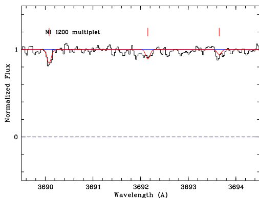
Fig. 1. The NI 1200 multiplet of the z_{\text{abs}}=2.0762 DLA in Q2206–199
