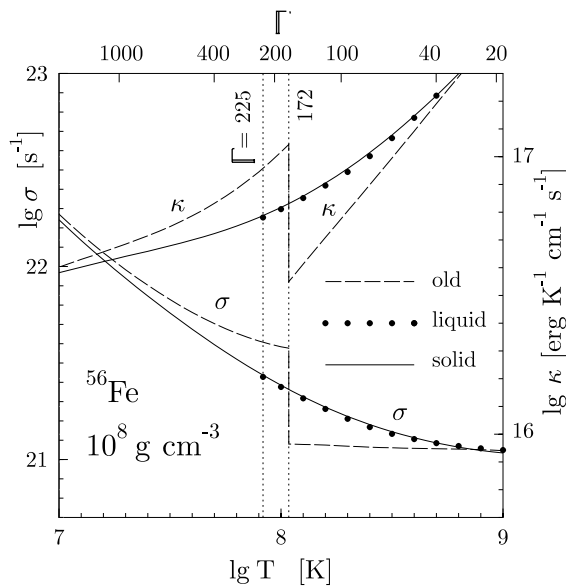
FIG. 2. Same as in Fig. 1 but for iron matter at density 10^8 \text{ g cm}^{-3} .
