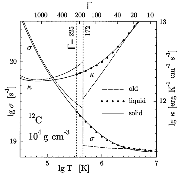
FIG. 1. Dependence of the electron electric (left vertical scale) and thermal (right vertical scale) conductivities of carbon plasma at density 10^4 \text{ g cm}^{-3} on temperature (lower horizontal scale) or ion coupling parameter (upper horizontal scale). Dashes are traditional results in ion liquid [3,7] and bcc crystal [4,6] for \Gamma_m = 172 . Solid line is the present multiphonon calculation in solid, extended artificially to high T ; show the present calculation with reduced structure factor in liquid at \Gamma \leq 225 . Vertical dotted lines correspond to \Gamma = 172 and 225.
