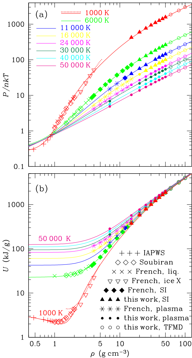
Fig. 4. Comparison of the data with the analytical fitted isotherms at high densities for the pressure normalized to the ideal atomic gas value, P/n_{\text{at}}k_B T (a), and for the internal energy U (b). Symbols show the data: the IAPWS table (Wagner & Pruß 2002, straight crosses); results of ab initio calculations by Soubiran & Militzer (2015) (empty diamonds); ab initio calculations by French et al. (2009) (oblique crosses for liquid, inverted triangles for ice X, filled diamonds for the superionic [SI] phase, asterisks for the plasma phase); and the results of our present ab initio calculations (filled triangles for the SI phase and filled dots for the plasma phase), supplemented with our TFMD calculations at \rho > 50 \text{ g cm}^{-3} (empty circles). Solid lines represent the present fit; the dotted line represents the fit of French & Redmer (2015) for ice X at T = 1000 K.
