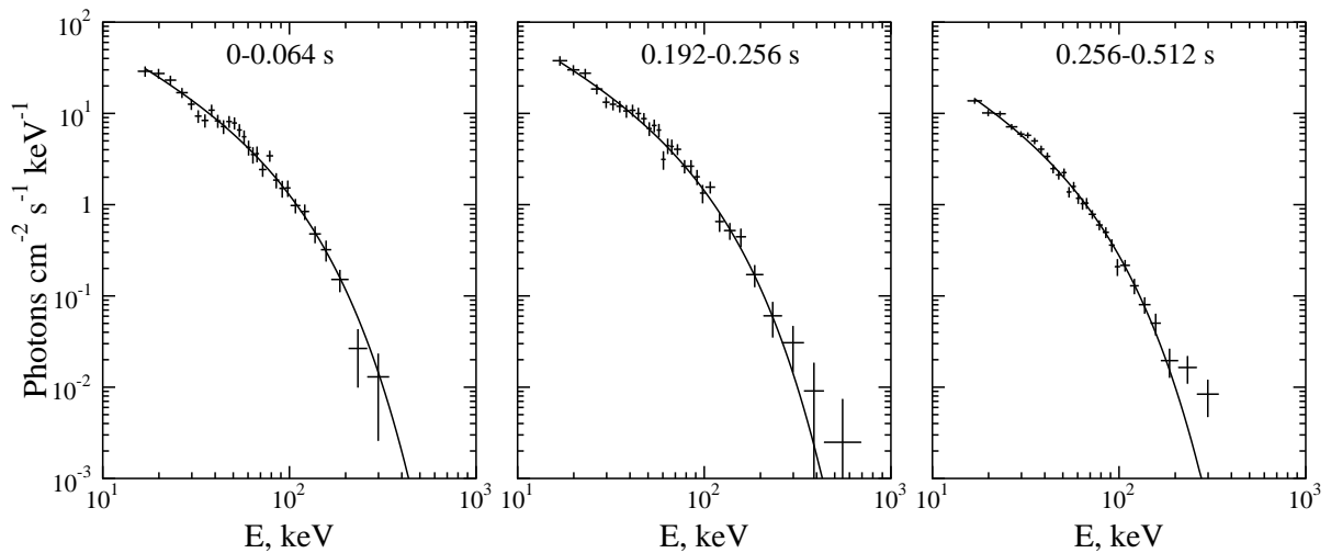
Fig. 5.7.— Energy spectra of the giant 980618d outburst.
