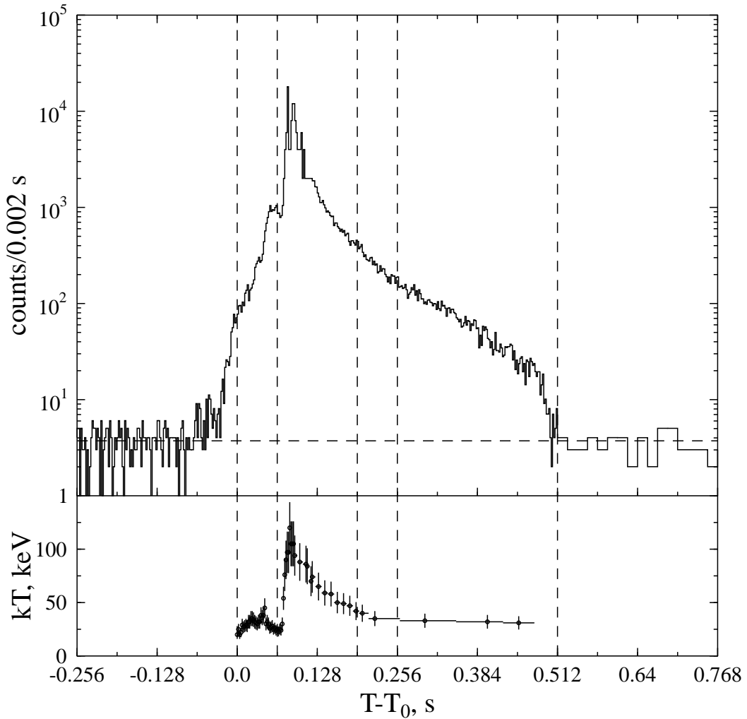
Fig. 5.6.— Extraordinarily intense 980618d outburst on 1998 June 18. Time history corrected for dead time (see Mazets et al. 1999a for details).
