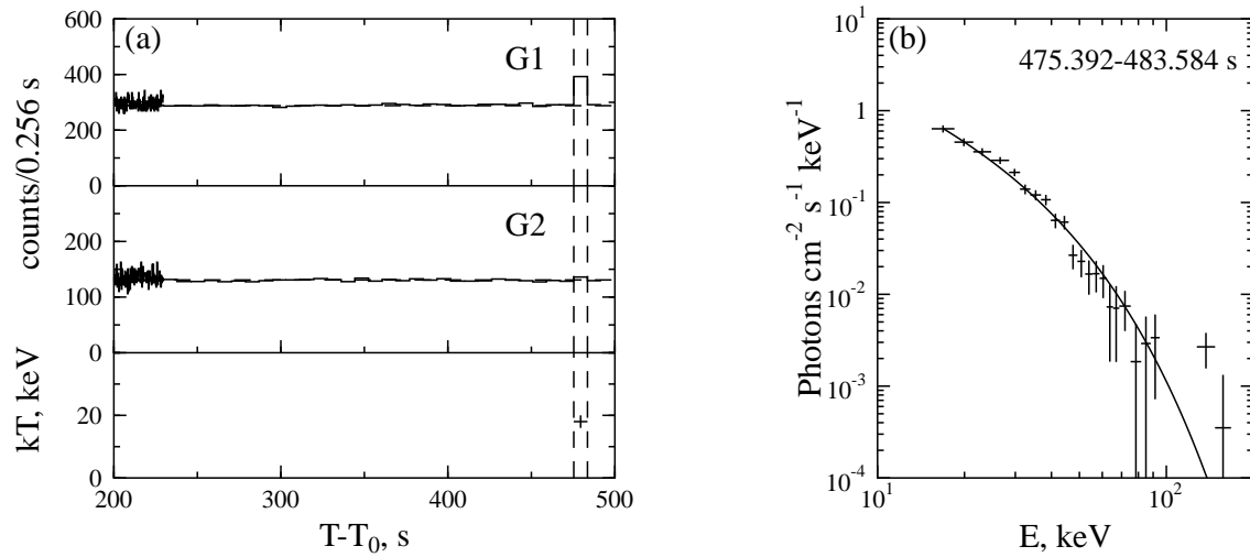
Fig. 5.2.— Burst 980617d (continued). See comments to Fig. 3.42.
