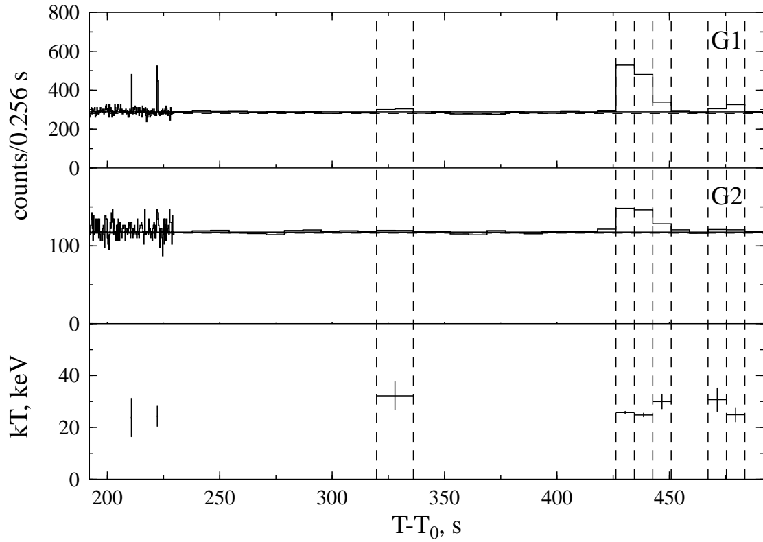
Fig. 3.56.— Event 981024. The final phase of the event. Unresolved cluster of soft bursts.
