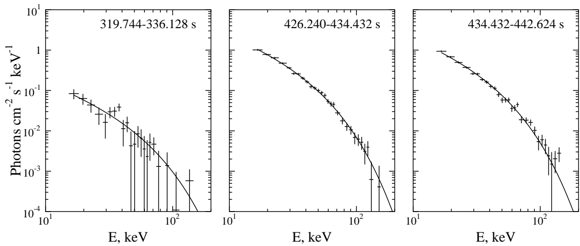
Fig. 3.57.— Event 981024. Energy spectra of the final phase.
