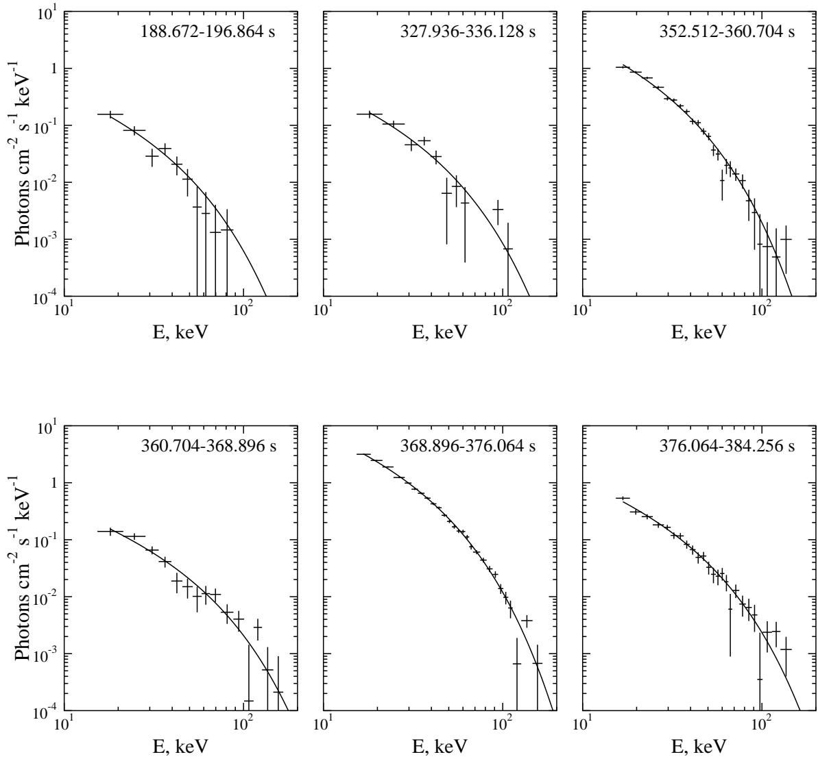
Fig. 3.43.— Energy spectra of the final phase of event 980901c.
