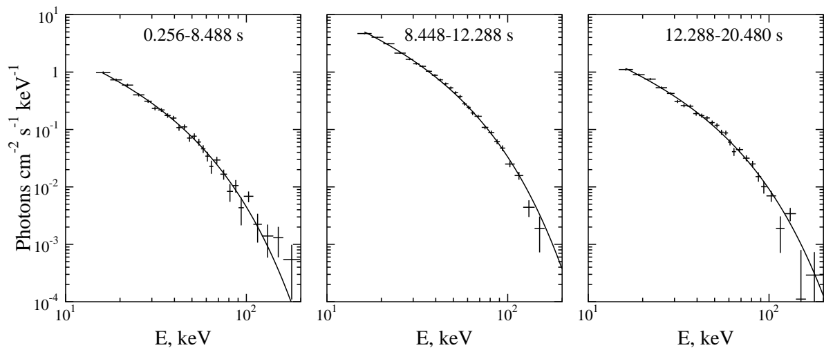
Fig. 3.10.— Energy spectra of the event 980530a accumulated in time intervals which include several separate bursts.
